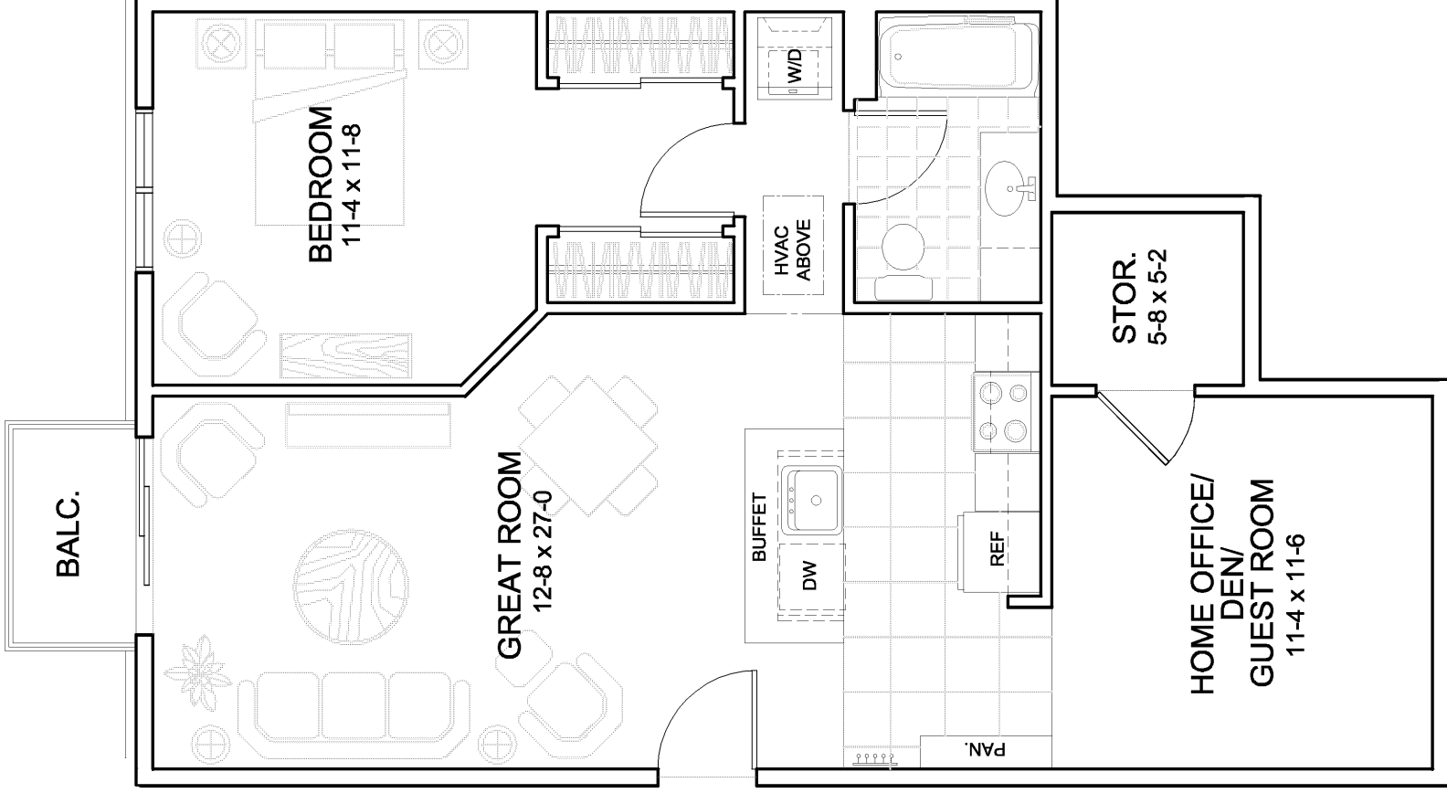
UNIT KEY PLAN (2nd & 3rd FLOORS)
