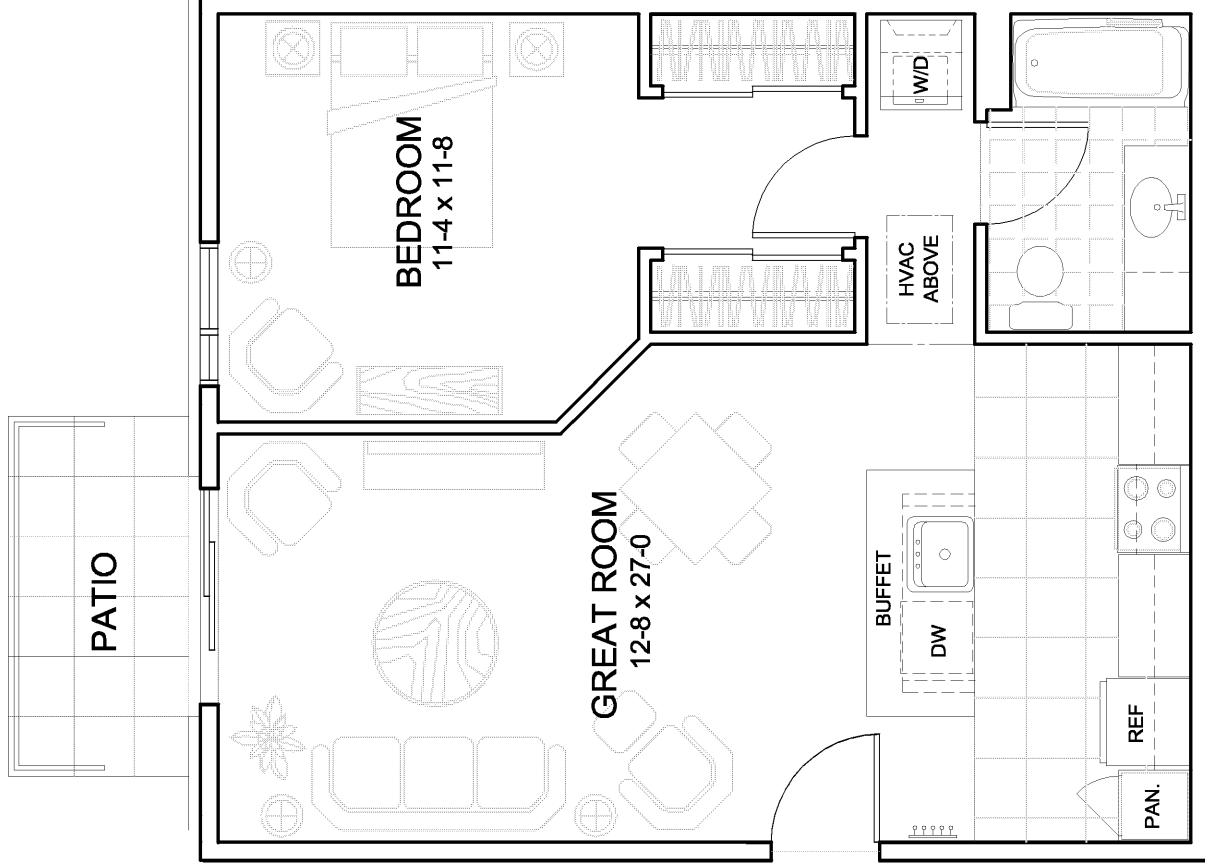
UNIT KEY PLAN (FIRST FLOOR ONLY)
