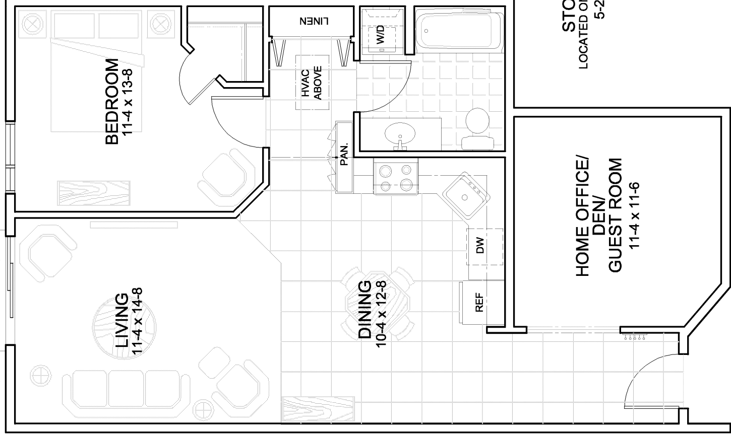
UNIT KEY PLAN (FIRST FLOOR ONLY)
