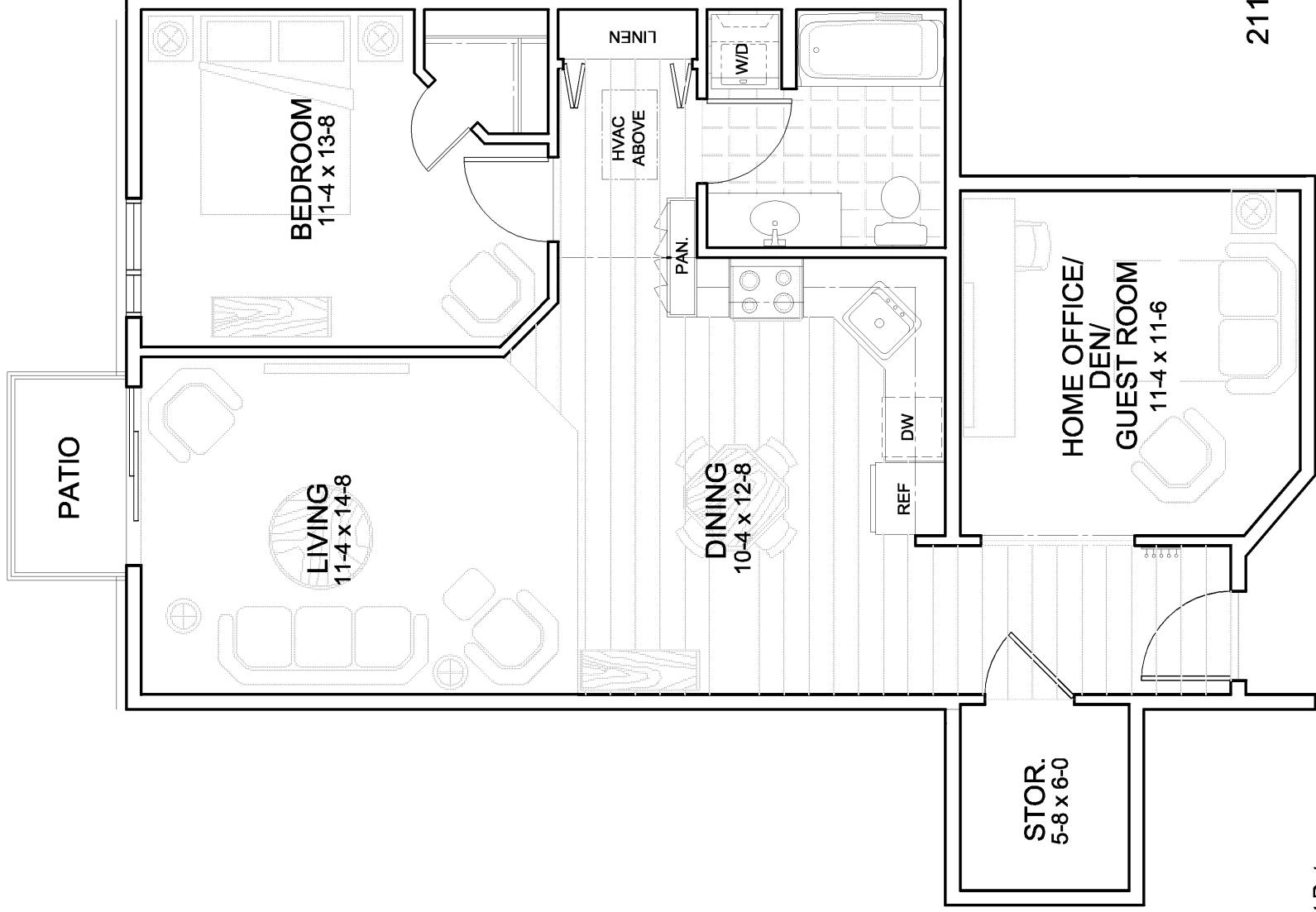
UNIT KEY PLAN (TYPICAL FLOOR)
