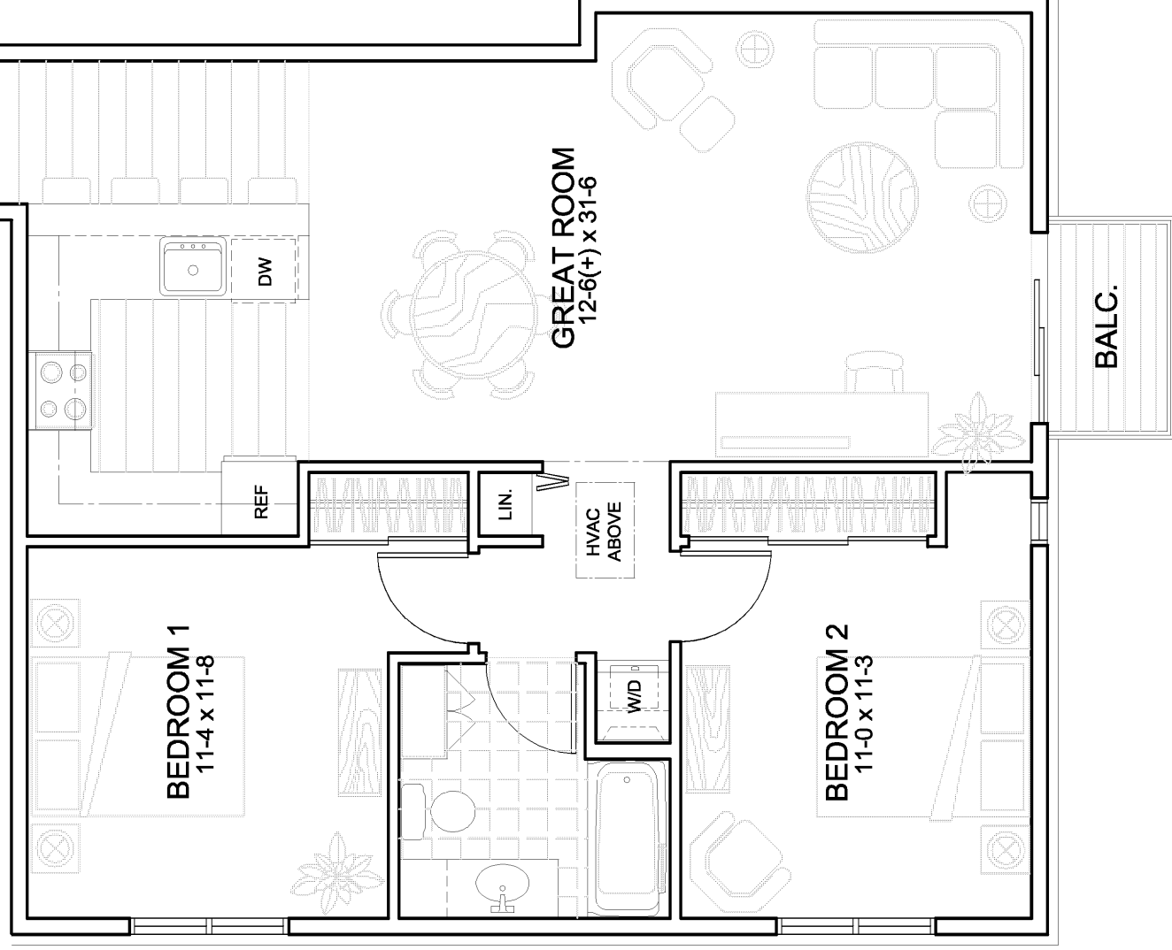
UNIT KEY PLAN (TYPICAL FLOOR)
